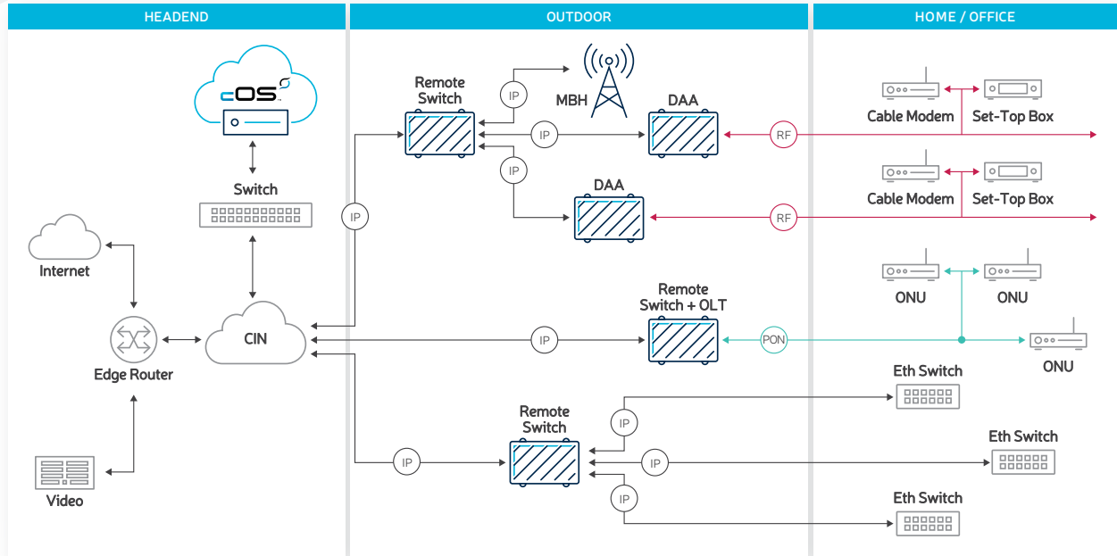
Deployment Diagram
